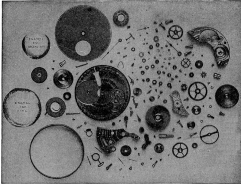
170 PARTS COMPOSE A 16 SIZE WATCH MOVEMENT. (A LITTLE MORE THAN \frac{1}{2} ACTUAL SIZE)
