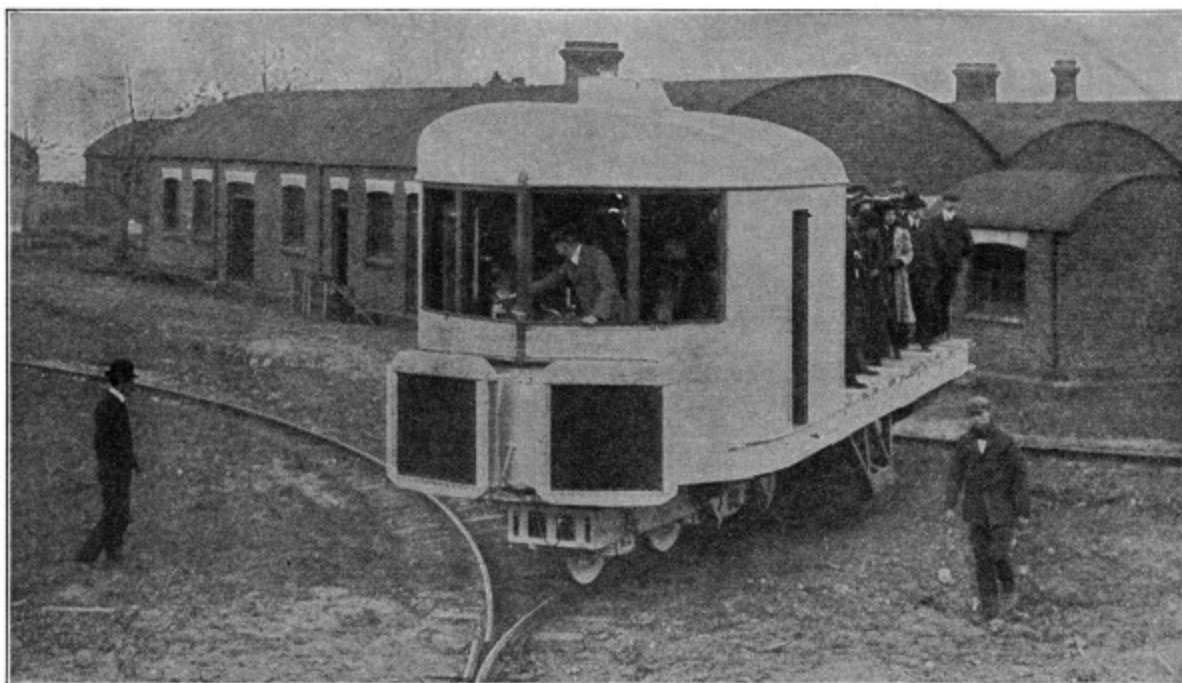
A MONORAIL GYROSCOPE CAR
