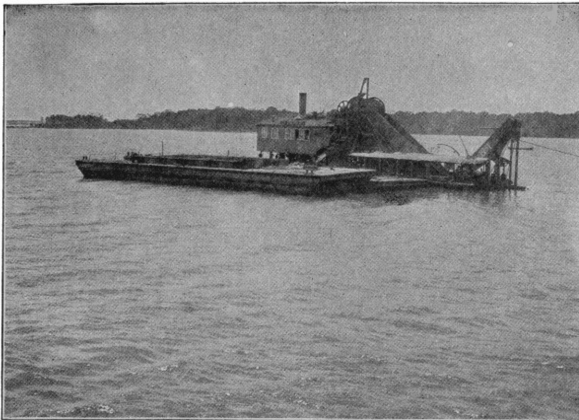
LADDER DREDGE, PANAMA CANAL
