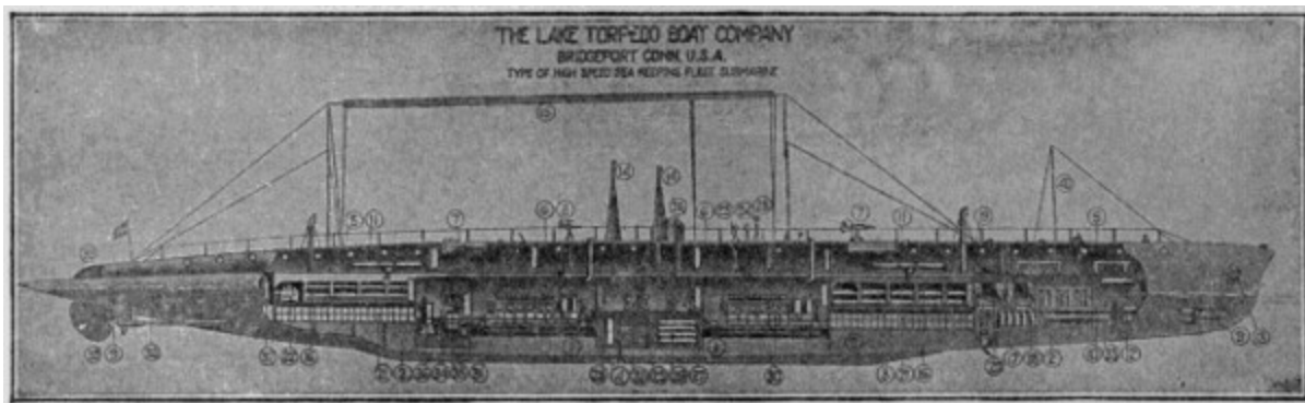
TYPE OF HIGH SPEED OCEAN-GOING SUBMARINE
