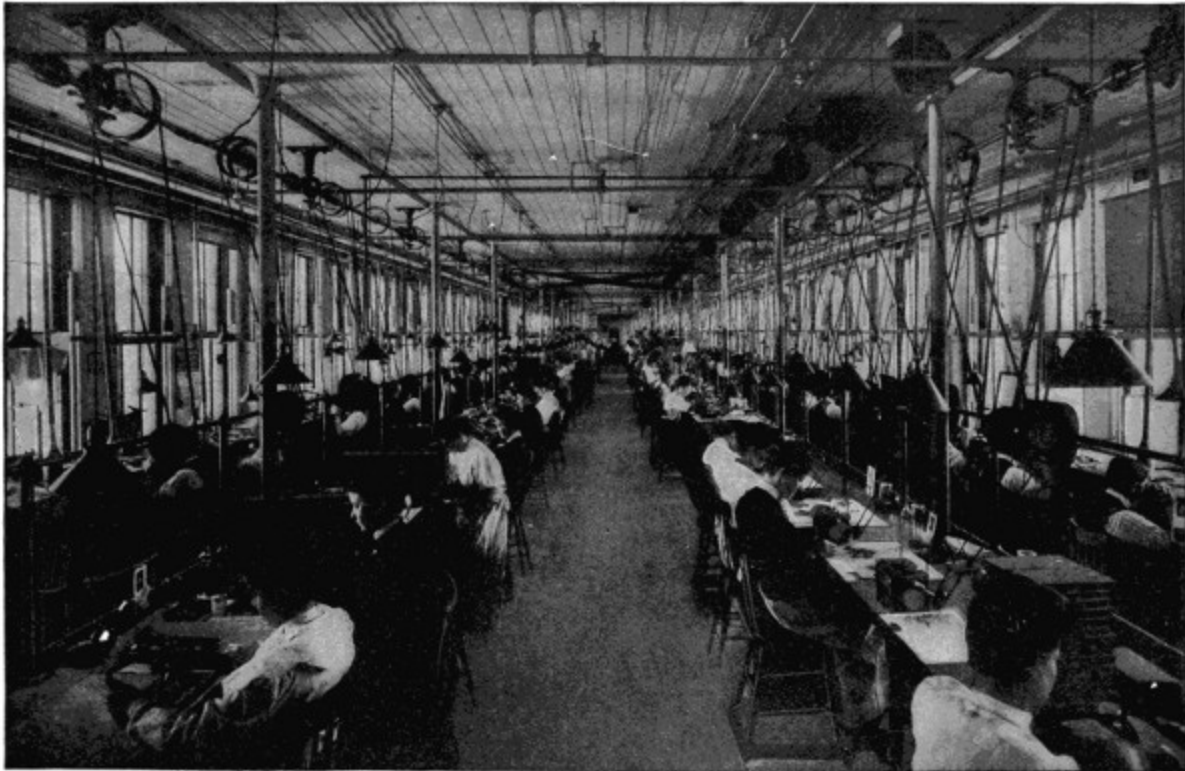
VIEW OF ESCAPEMENT MAKING DEPARTMENT
